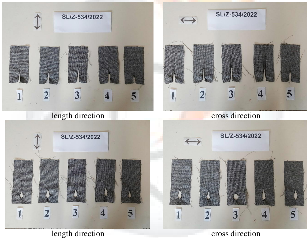
Figure 6. Appearance of the sample after the small burner test – HEGL01
