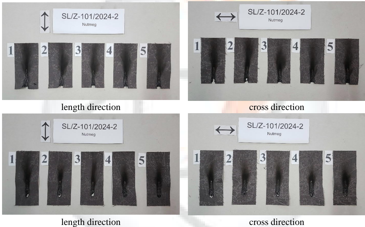
Figure 6. Appearance of the sample after the small burner test – Nutmeg/212275-14
