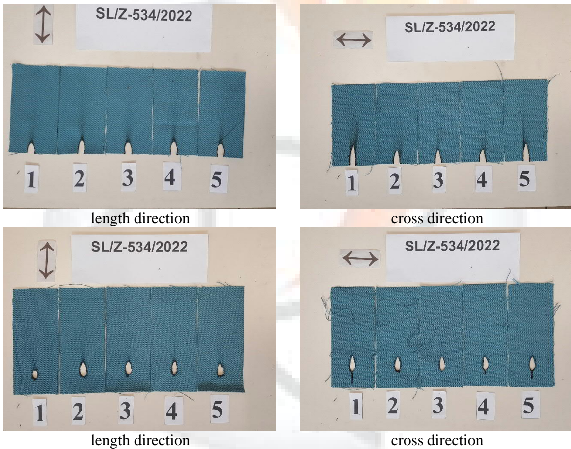
Figure 6. Appearance of the sample after the small burner test – HOOC02
