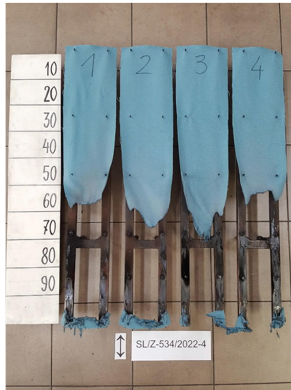
Figure 3. Appearance of the sample 2 after the test – HOOC02 – length direction
